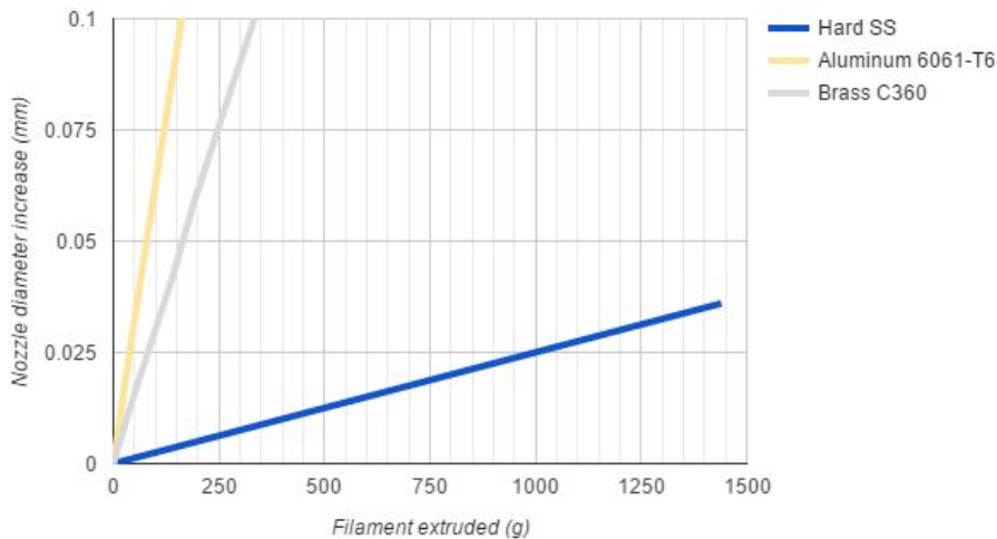
Nozzle size increase from extruding carbon fiber
